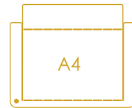
Tray (A4 horizontal) 400mm X 250mm X 75mm 4mm bend: /4 FLD/TRAY/01
