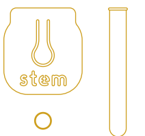
Vase 65mm X 65mm X 150mm 4mm bend: /4 FLD/STEM/00
